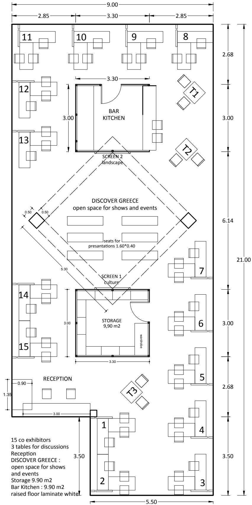
PLAN - STAND GNT0 - BARCELONA scale 1/100
